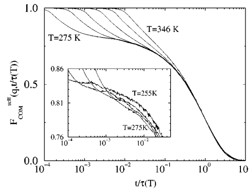
FIG. 4. \alpha scaling for the c.o.m. self-correlation function for different T at q = 13 nm -1 , the position of the first minimum of S_{c.o.m.}(q) . The main plot shows, from right to left, T=346, 318, 305, 291, 281, and 275 K. The inset shows the region around the plateau for T=275, 266, 260, and 255 K.
